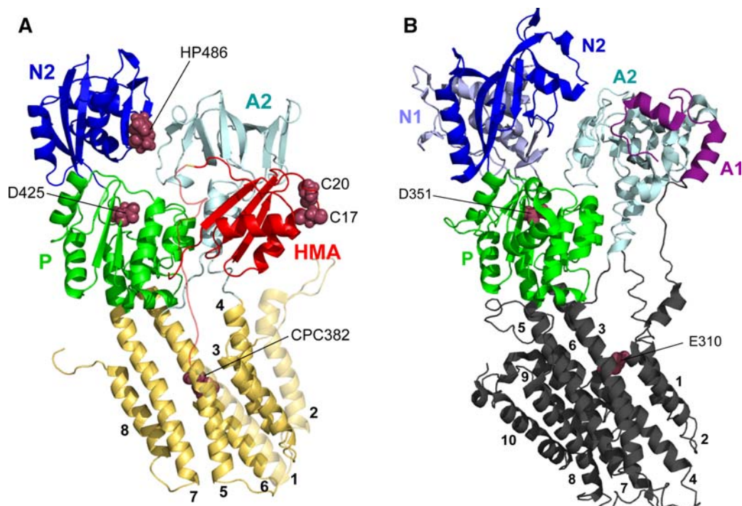
Fig. 4 Comparison of the CopA model (Model-2) with the structure of Serca1. a CopA model with the HMA-domain colored in red, the A2-domain in grayish blue, the N2-domain in dark blue, the P-domain in green, and the transmembranous domain in ochre. TM1 and TM2 and their connecting loops are displayed in a lighter shade to indicate the spatial uncertainty. b Structure of Serca1 (PDB entry 1IWO). The A1-domain is
